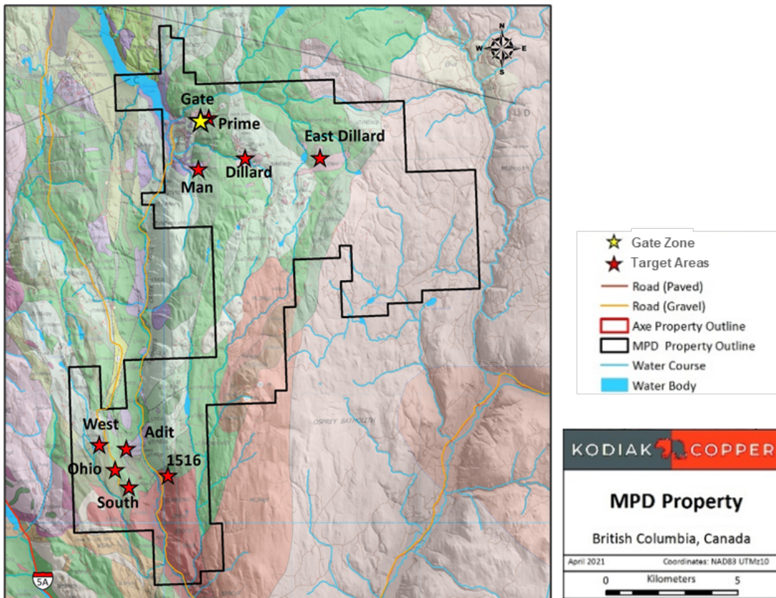
Figure 2: Geology and Copper Porphyry Zones, MPD Property.
