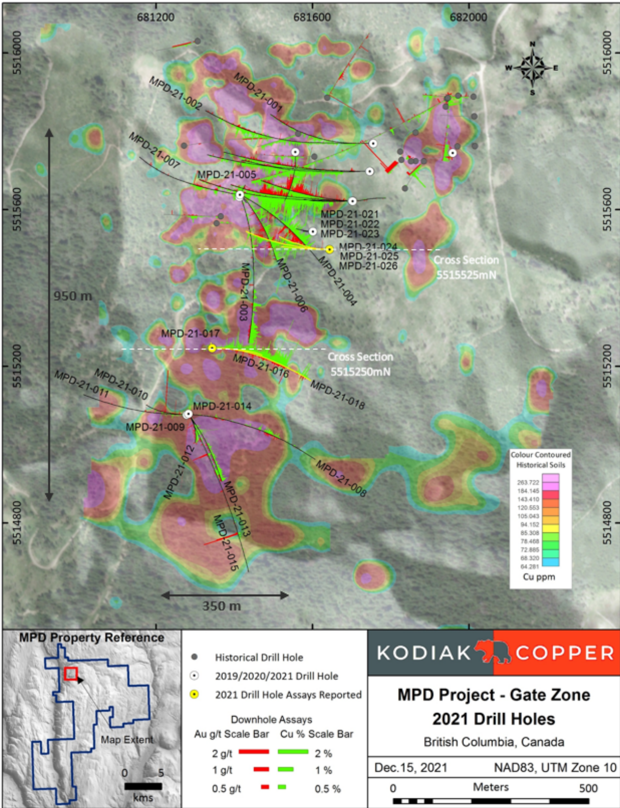
Figure 1: Gate Zone plan map showing all 2021 drilling with assay results to date. Background is contoured historic copper-in soil data. Porphyry-related mineralization at Gate has been traced down to 850 m depth, across a width of 350 m (east-west) and over 950 m in length (north-south)
