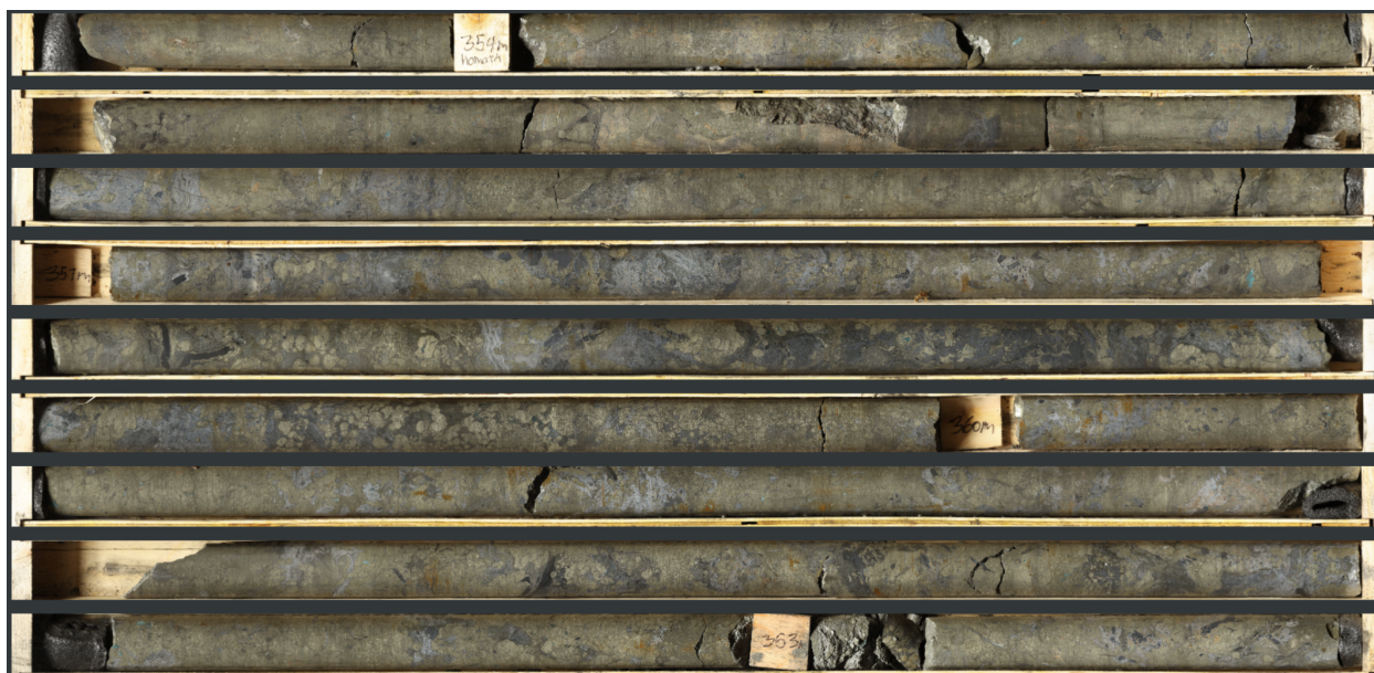
Photo 3: High resolution core scanning image of sphalerite-pyrite-galena-siderite breccia mineralization in NB23-020 (353.7 m to 363.4 m).
