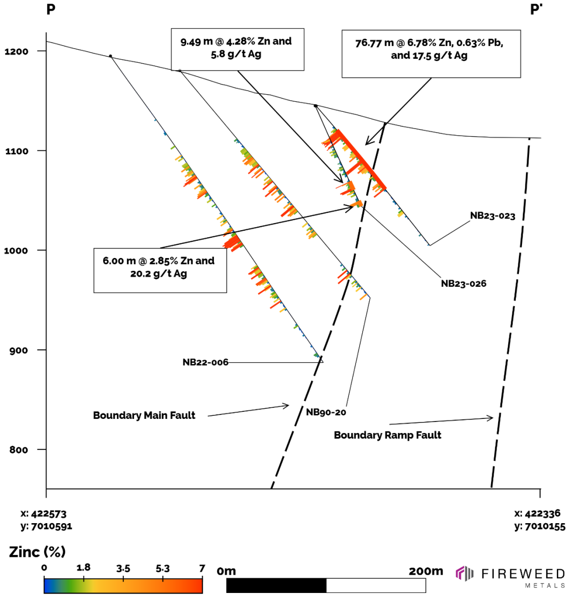
Cross Section P-P' — Including analytical results from Hole NB23-023 and NB23-026
