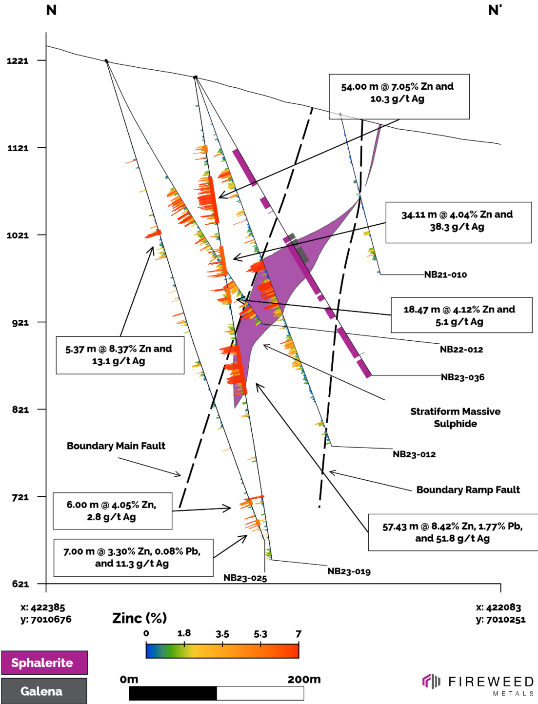
Cross Section N-N' — Including Holes NB23-019 and NB23-025.
