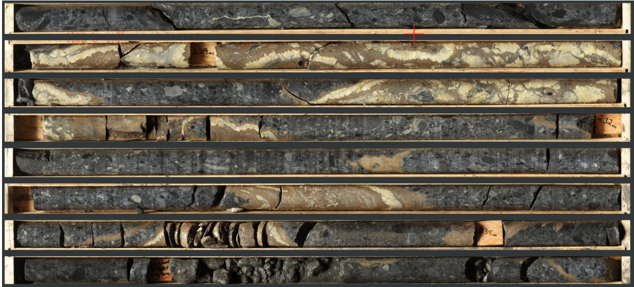
Photo 2: High resolution core scanning image of sphalerite-pyrite-siderite vein mineralization in NB23-027 (227.5 m to 235.9 m).
